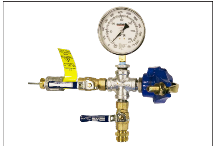
Sure-Off Tester
