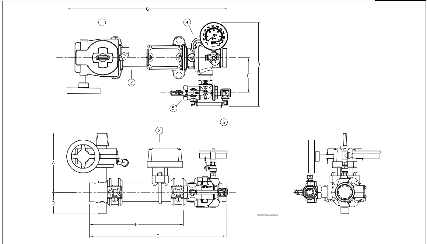
Model FCA Dimensions (Refer to Table D)
