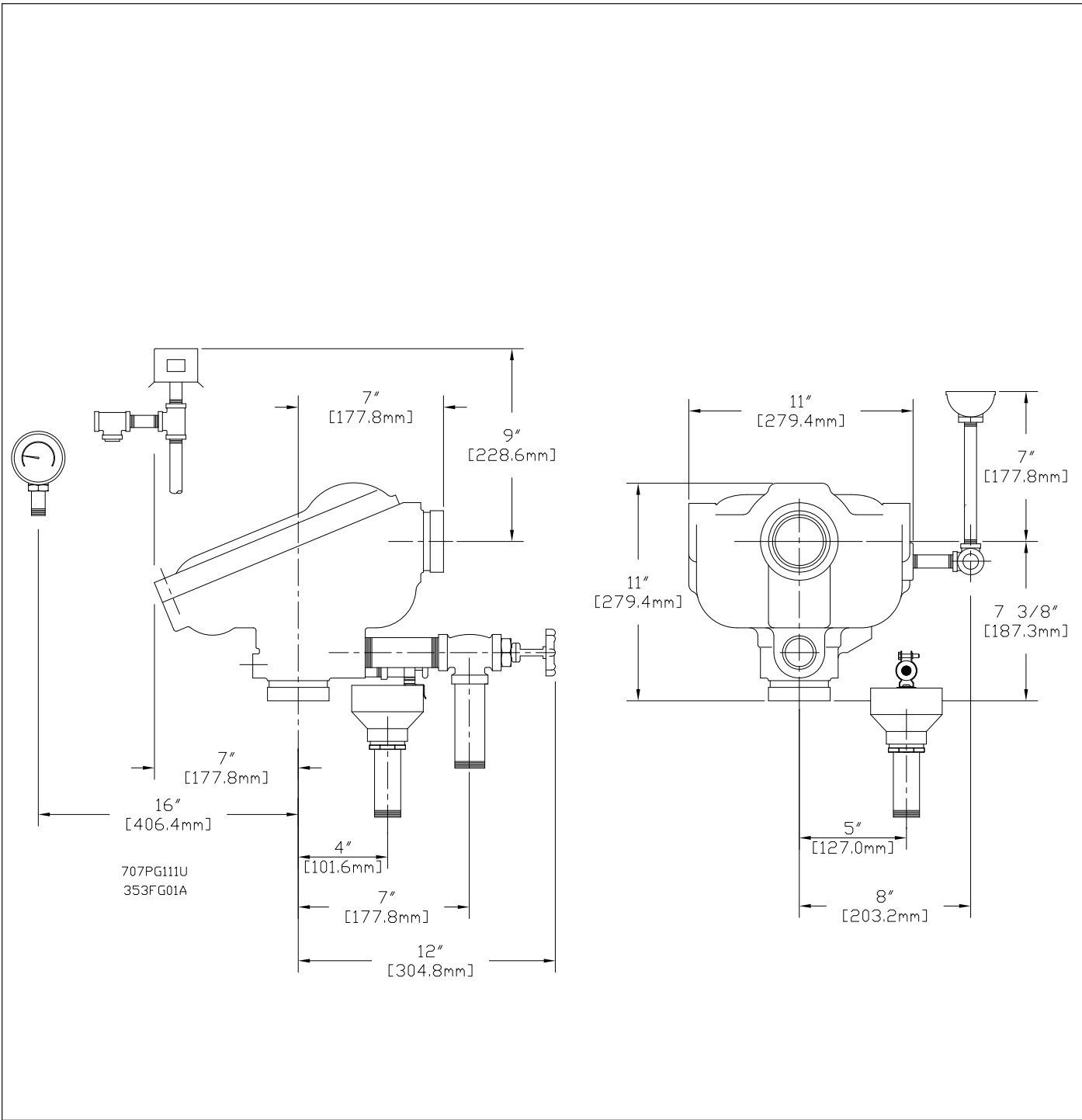
Fig. 1 - Installation Dimensions in Inches (mm)
