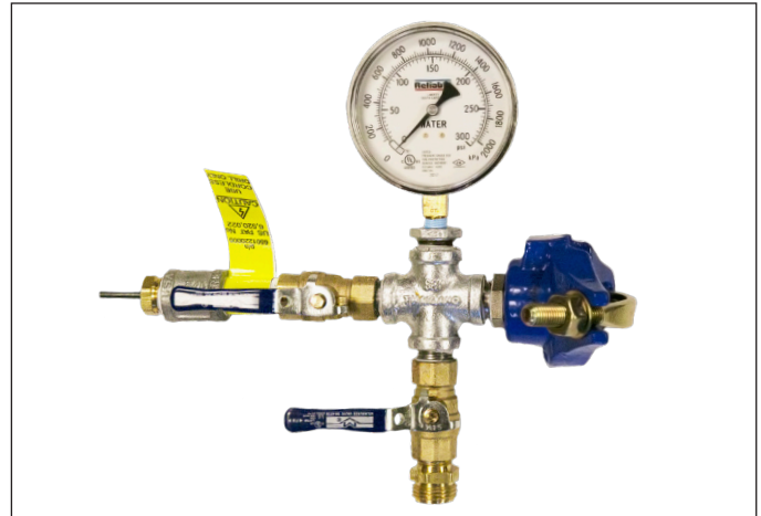
Sure-Off Tester
