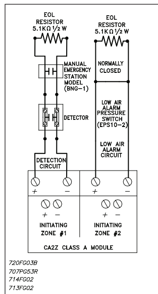
Class b Wiring Figure 3
