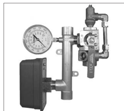
Fig. 4 Base Trim with TestANDrain® Valve & Pressure Relief Kit
