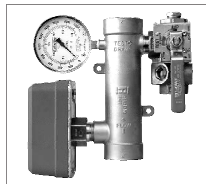
Fig. 3 Base Trim with TestANDrain® Valve
