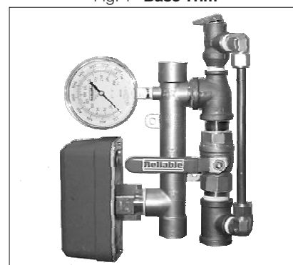
Fig. 2 Base Trim with Pressure Relief Kit
