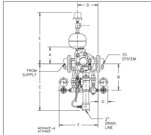
Horizontal Constant Trim – Front Elevation
