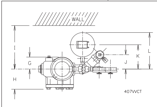
Vertical Variable Trim – Front Elevation
