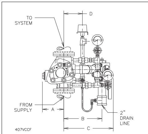
Vertical Constant Trim – Front Elevation
