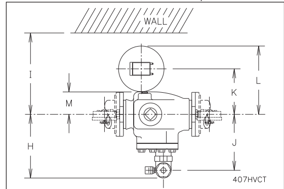
Horizontal Variable Trim – Front Elevation
